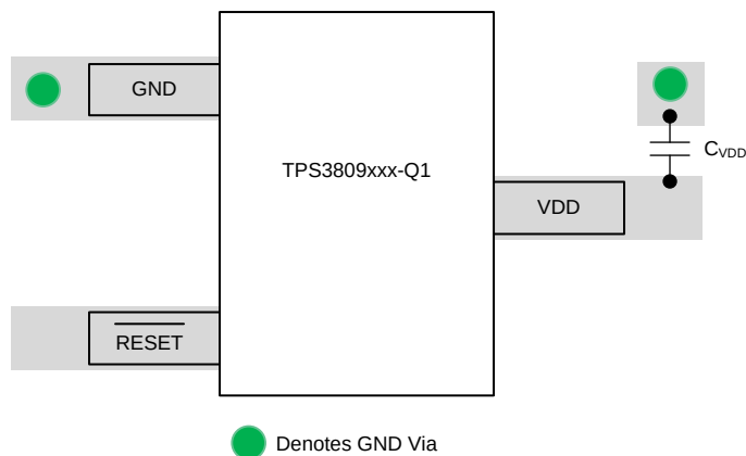
Figure 11. Layout Example
