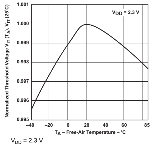
Figure 10. Normalized Input Threshold Voltage vs Free-Air Temperature at V DD
