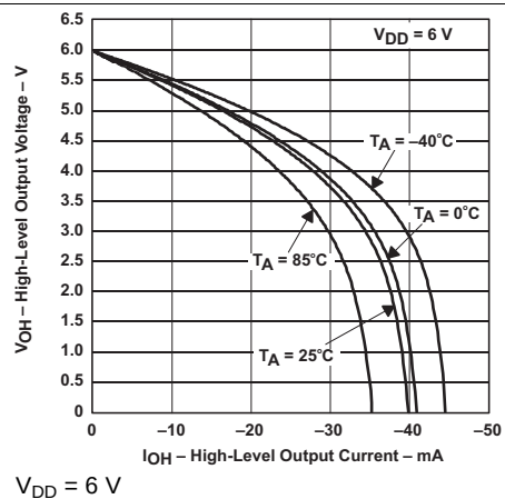
Figure 4. High-Level Output Voltage vs High-Level Output Current
