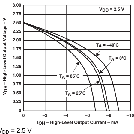
Figure 5. High-Level Output Voltage vs High-Level Output Current
