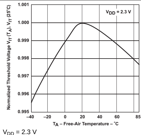
Figure 6. Normalized Input Threshold Voltage vs Free-Air Temperature at V_DD
